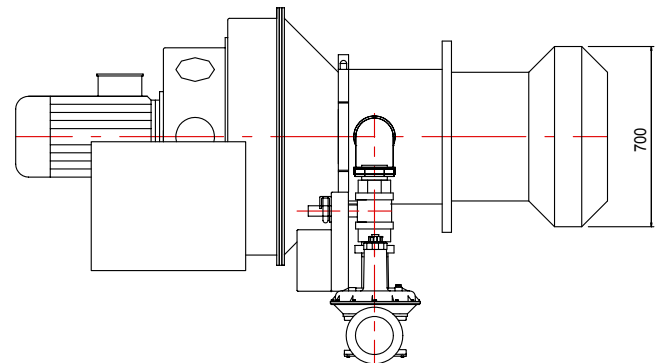
BURNER MOUNTING DETAIL
