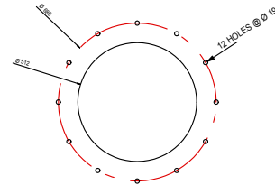
BURNER MOUNTING DETAIL
